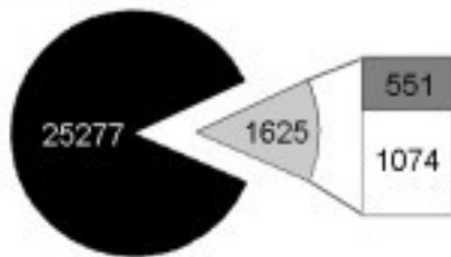
Valproic Acid
