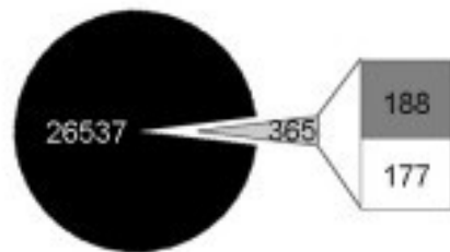
HDAC3 KD
