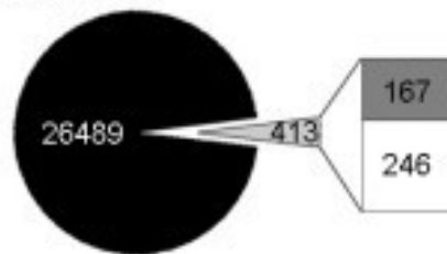
HDAC2 KD
