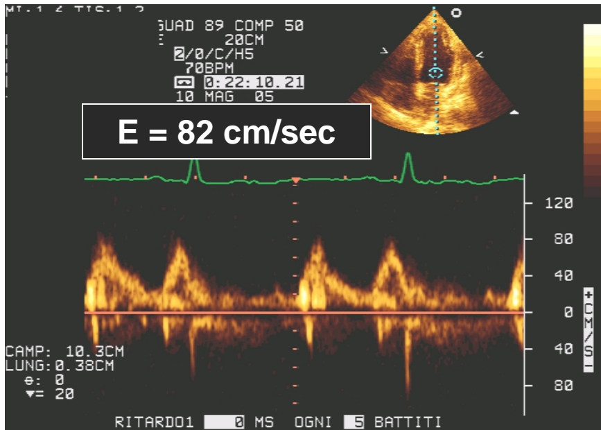
Mitral flow
