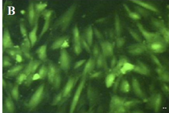
NO/Ar-Containing liposome In the absence of homoglobin
