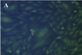
NO/Ar-saturated solution In the absence of homoglobin
