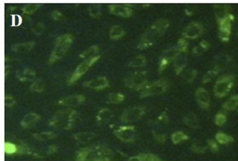
NO/Ar-saturated solution In the presence of homoglobin
