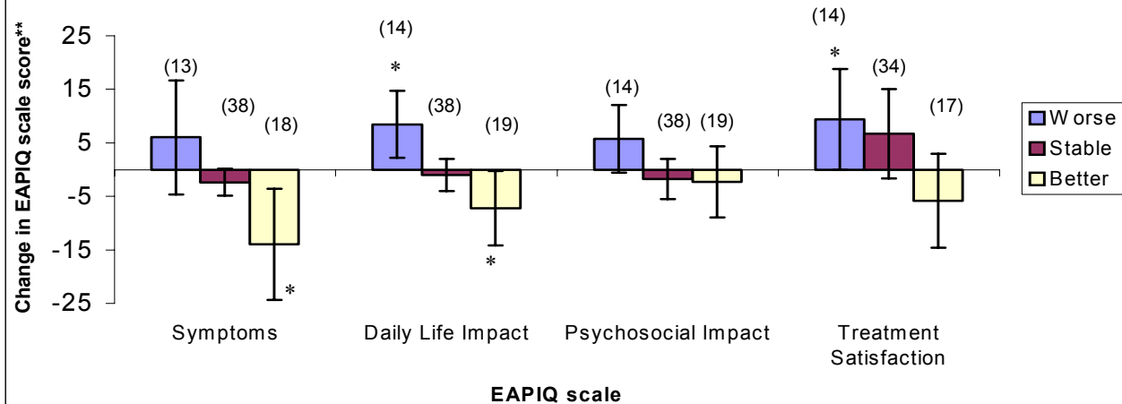
Figure 5. Responsiveness: change over time in EAPIQ scales by change in eye allergies
