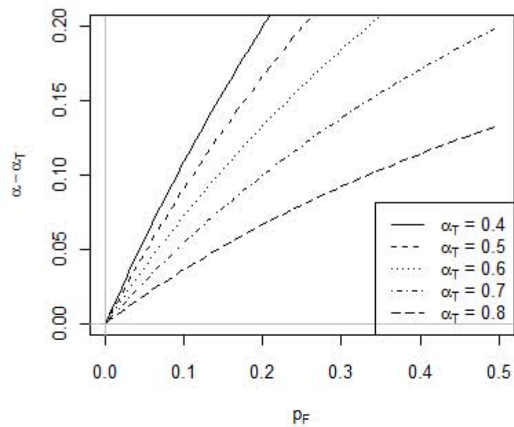
(a) p_R = 0, m+ - m- = 5
