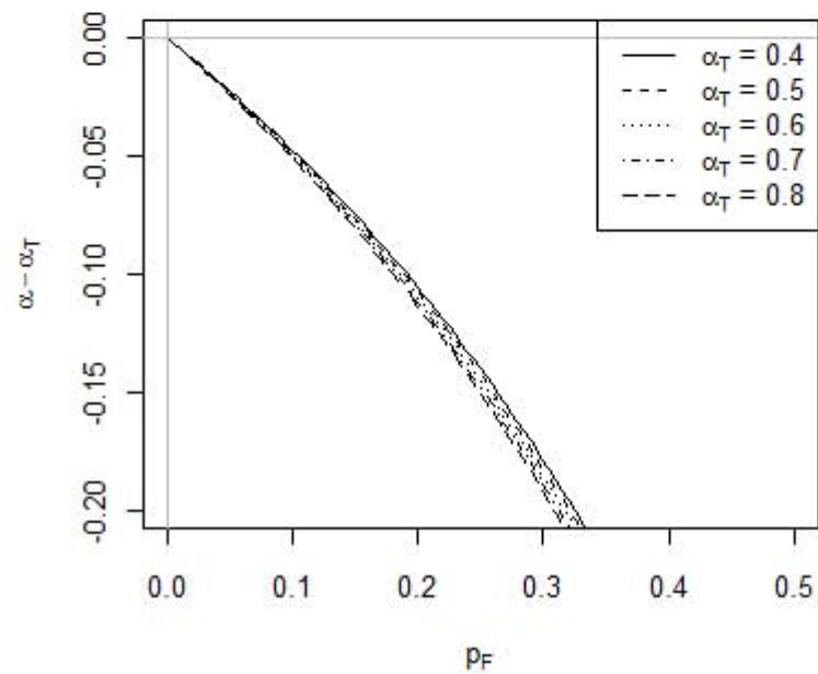
(c) p_R = 0, m+ - m- = 1
