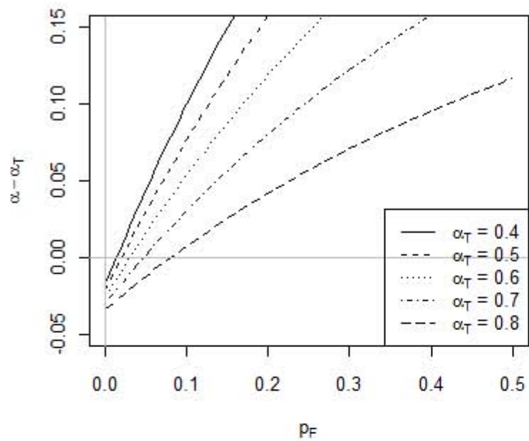
(b) p_R = 0.1, m+ - m- = 5
