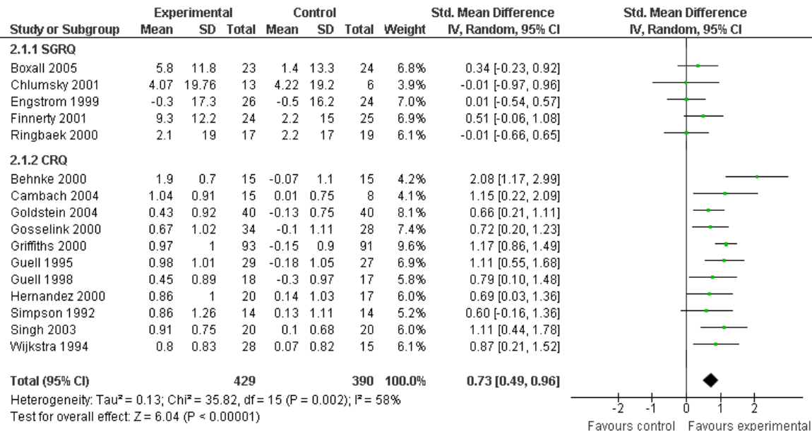
Figure 1: Pooled Estimate in SMD Units
