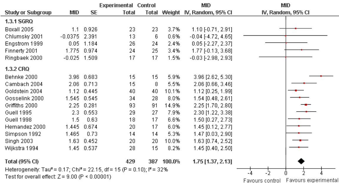
Figure 2: Pooled Estimate in MID Units
