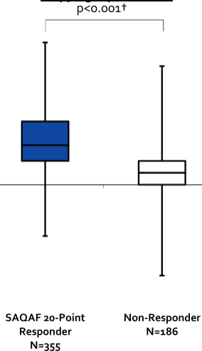
Mapping Equation #2#
