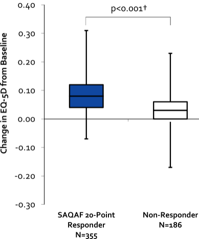
Mapping Equation #1*
