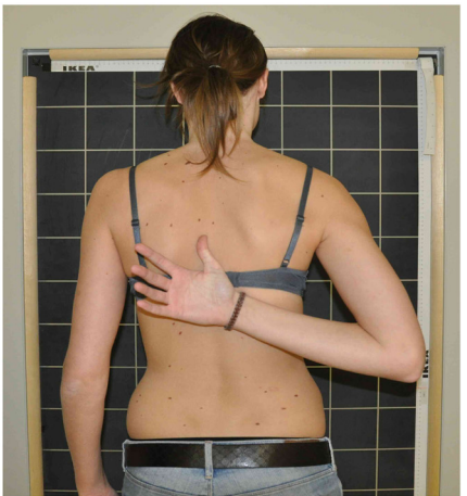
Endorotation.
