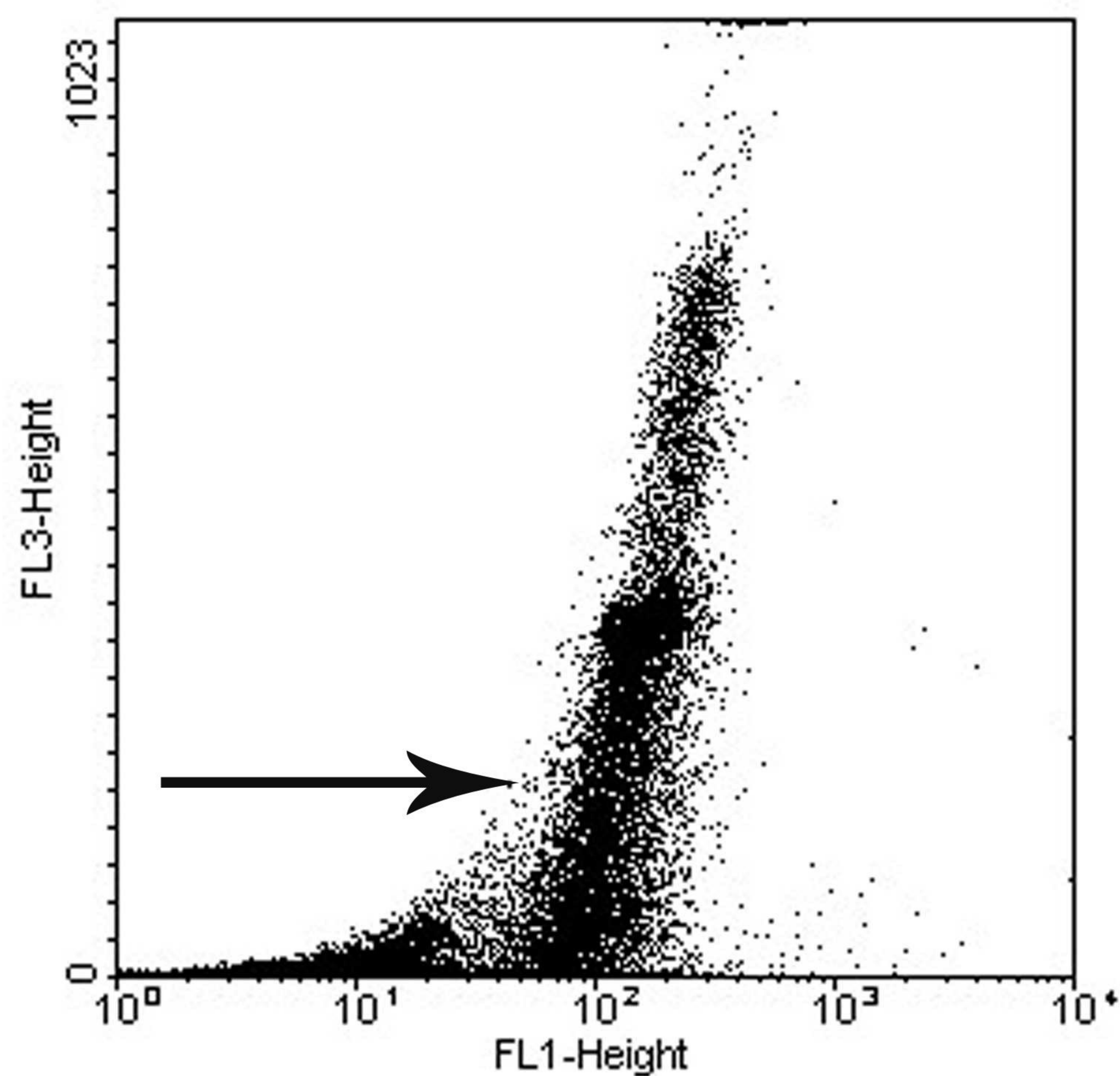
Gc-5spg CAP 200 \mu M, 48 hour
