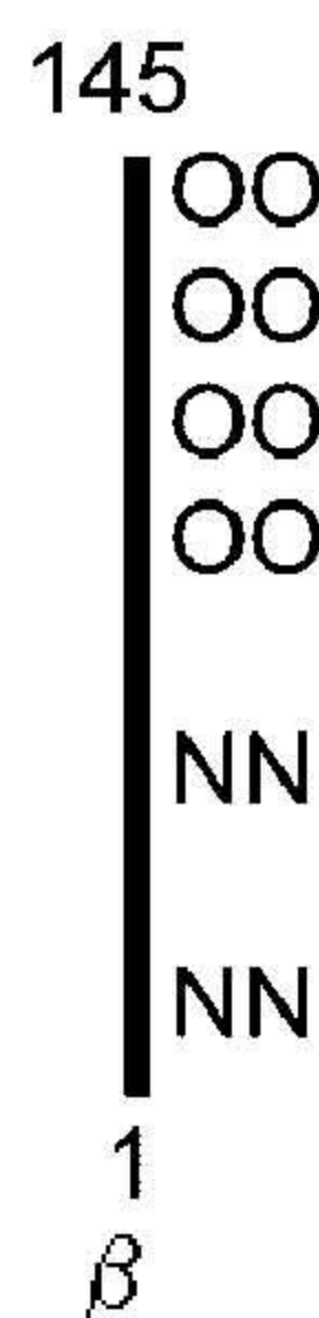
Nicked hyperglycosylated hCG free \beta missing \beta CTP
