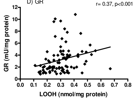
D) GR
