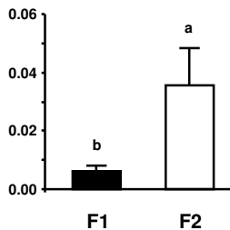
SELP
