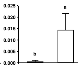
PLAUR
