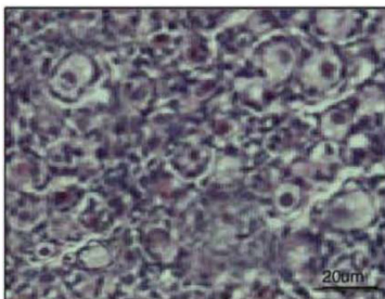
Calphostin group
