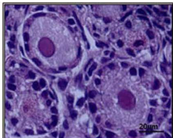
Blank control
