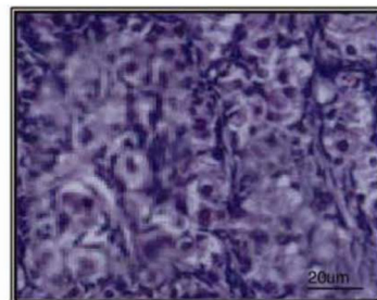
LY294002 group
