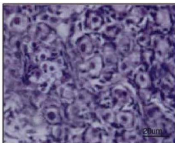
PD98059 group
