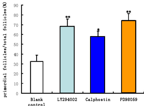
Calphostin group
