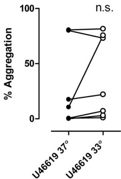
C U46619 10 \mu\text{M}
