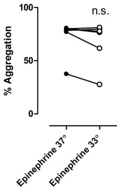
A Epinephrine 10 \mu\text{M}
