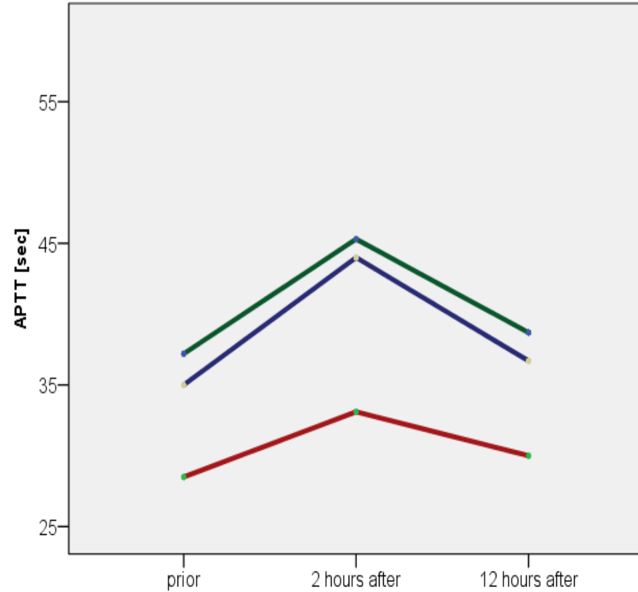
Rivaroxaban
