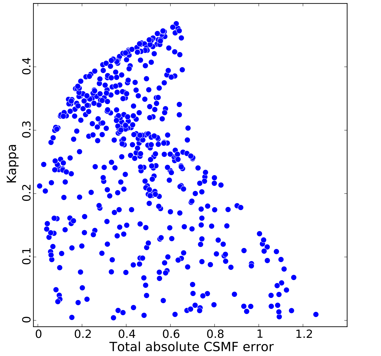
Kappa versus total absolute CSMF error for method 1
