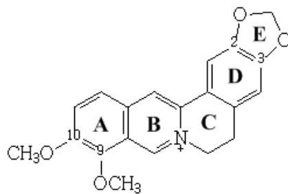
BBR: berberine
