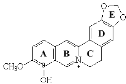
M1: berberrubine
