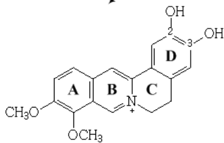
M3: demethyleberberine
