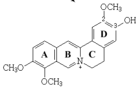
M4: jatrorrhizine
