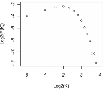
A: Random Network (In-degree)
