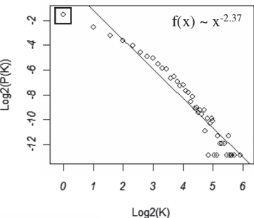
C: Real Network (In-degree)
