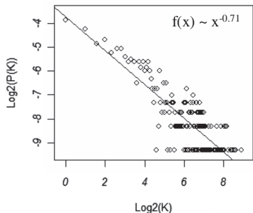
D: Real Network (Out-degree)
