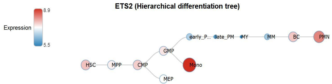
Figure S1. The hierarchical differentiation tree of relationship between ETS2 expression level and hematopoietic cell differentiation. HSC: Hematopoietic stem cell; MPP: Multipotential progenitors; CMP: Common myeloid progenitor cell; GMP: Granulocyte monocyte progenitors; MEP: Megakaryocyte-erythroid progenitor cell; early-PM: Early Promyelocyte; late-PM: Late Promyelocyte; MY: Myelocyte; MM: Metamyelocytes; BC: Band cell; PMN: Polymorphonuclear cells; Mono: Monocytes.
