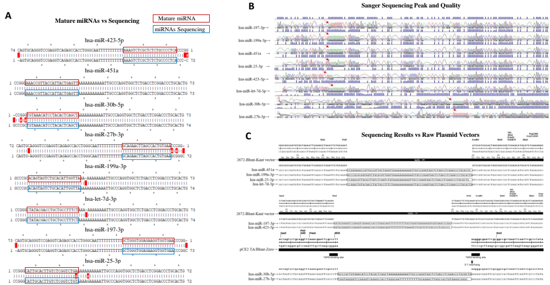
Additional file 6: Figure S5. The sequencing information of 7 potential miRNA biomarkers and reference miRNA. A. Alignment of mature miRNAs and sequencing results; B. Sanger sequencing peak and quality; C. Schematic diagram of cloning RT-qPCR products to plasmid vectors.
