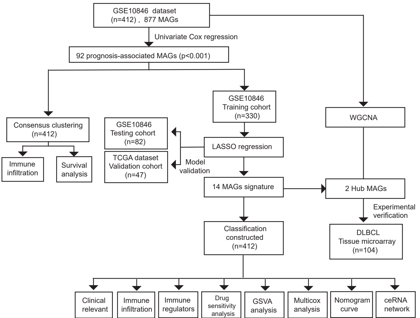
Additional file 1: Figure S1. Flow chart of the data analyzing process. The GSE10846 dataset was randomly divided (4:1 ratio) into a training cohort (n=330) and a testing cohort (n=82).
