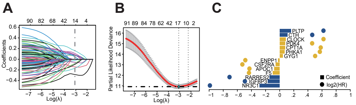
Additional file 5: Figure S5. LASSO regression analysis revealing the minimum criteria ( A, B ) and coefficients ( C ). Blue represented the coefficient greater than 0.1, and yellow represented the coefficient less than 0.1.
