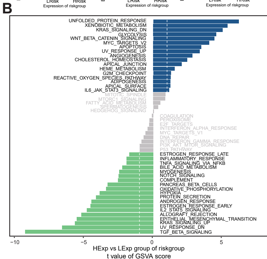
Additional file 7: Figure S7. Prediction of drug sensitivity and signaling pathways in high- and low-risk groups. (A) Sensitivity analysis of common therapeutic drugs in patients of two groups. (B) GSVA analysis for differentially expressed signaling pathways between two groups.
