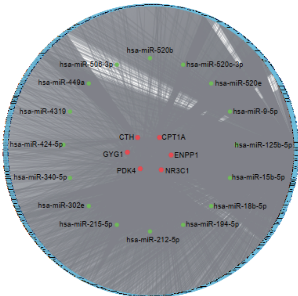
Additional file 8: Figure S8. The ceRNA network associated with the model genes. The red dots represent mRNAs, the green dots represent miRNAs and the blue dots represent lncRNAs.
