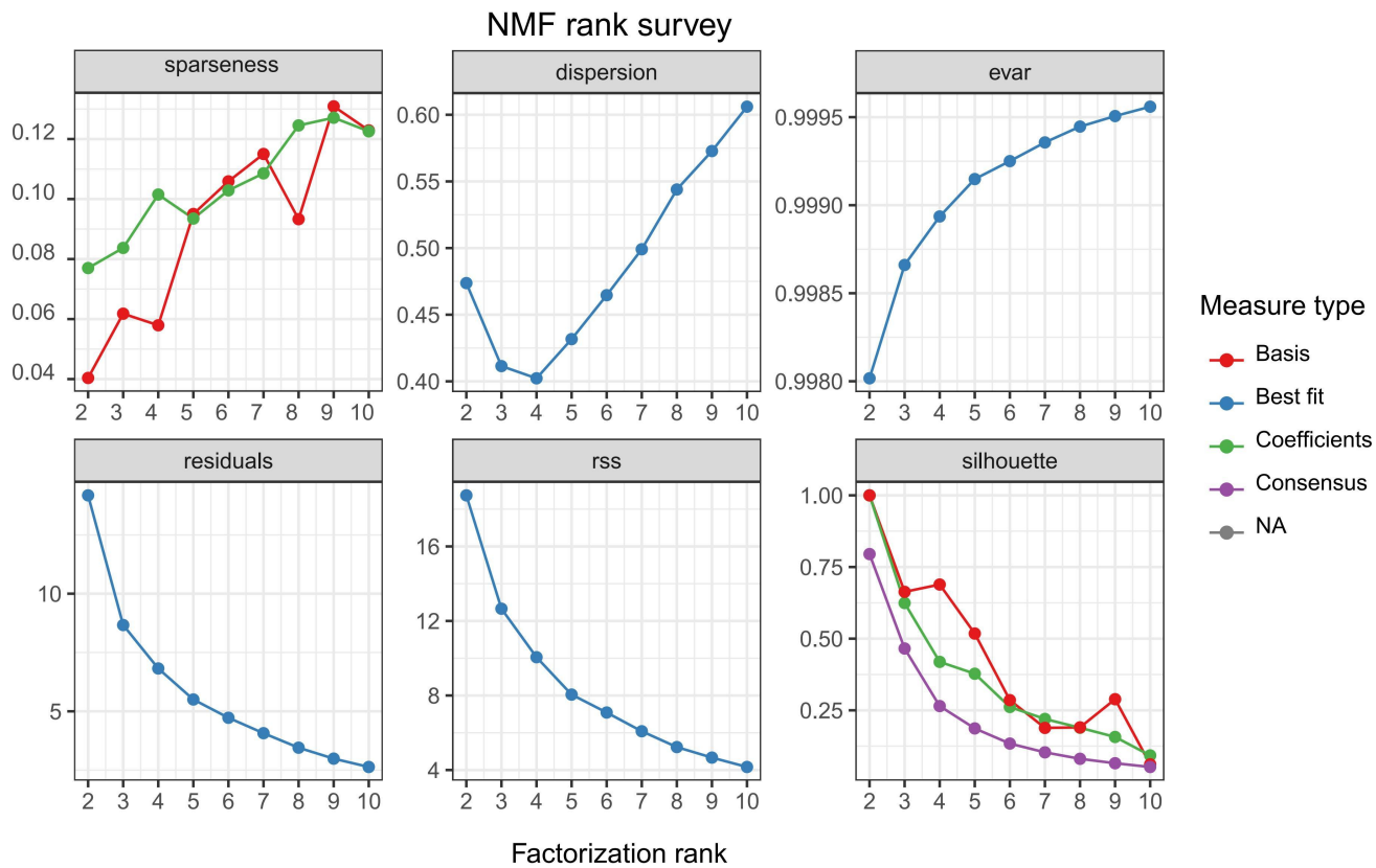
Supplementary Figure 1. The NMF rank survey at a rank of 2 to 10.
