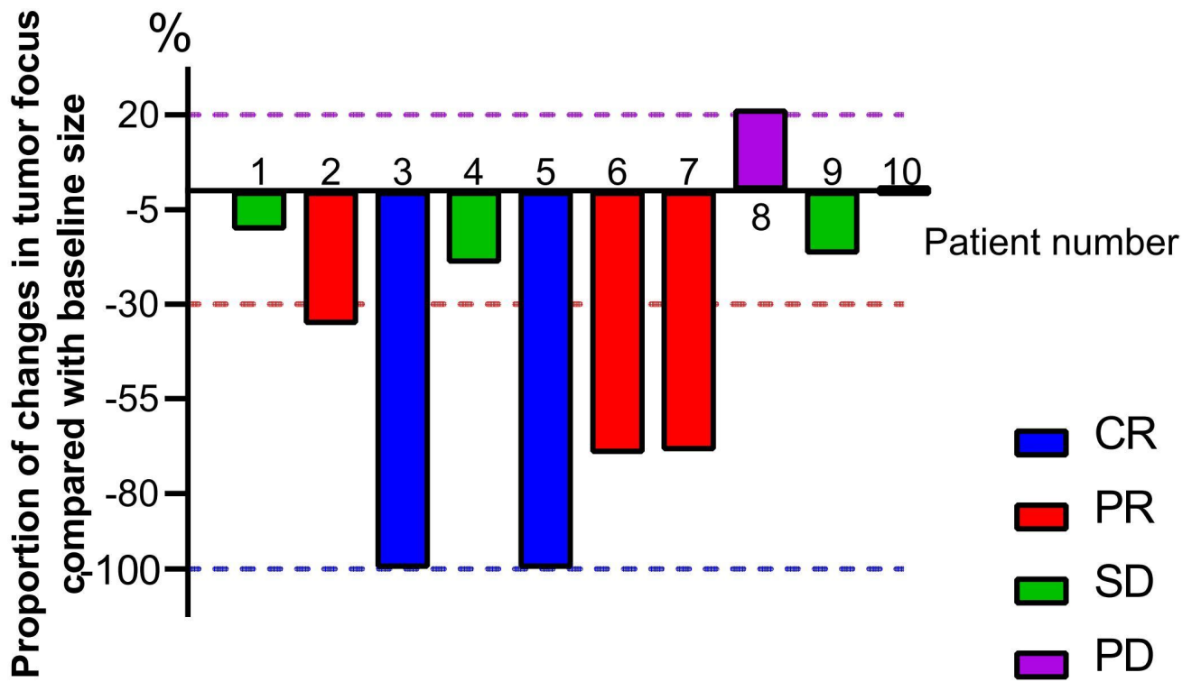
Supplementary Figure 3. The ten patients' best response evaluation in our independent LUSC cohort according to response evaluation criteria in solid tumours (RECIST, v1.1).
