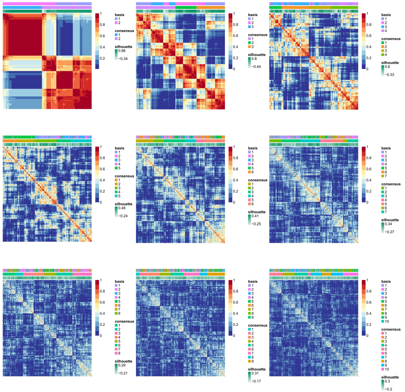
Supplementary Figure 2. All heatmaps of the training set with the number of clusters ranged from 2 to 10.
