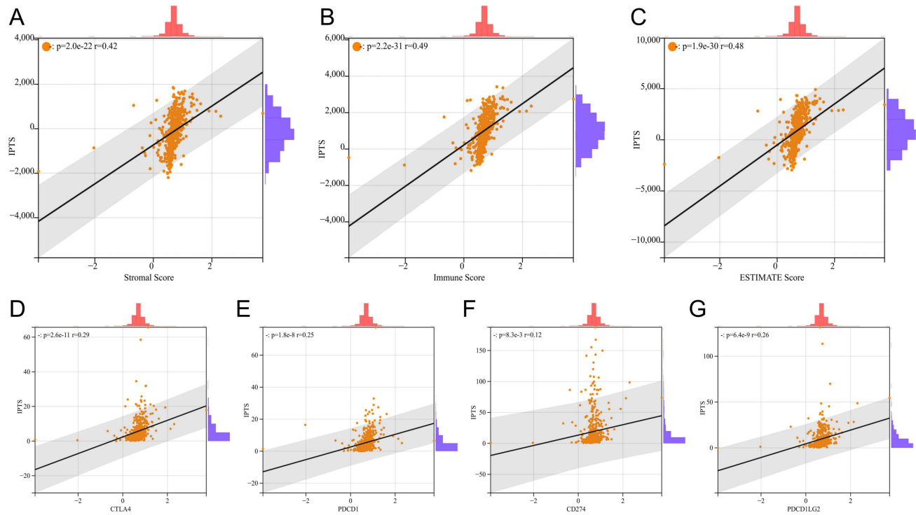
Supplementary Figure 4. Correlation analysis between IPTS and (A) stromal score, (B) immune score, (C) ESTIMATE score, (D) CTLA4 TPM value, (E) PDCD1 (PD-1) TPM value, (F) CD274 (PD-L1) TPM value, and (G) PDCD1LG2 (PD-L2) TPM value.
