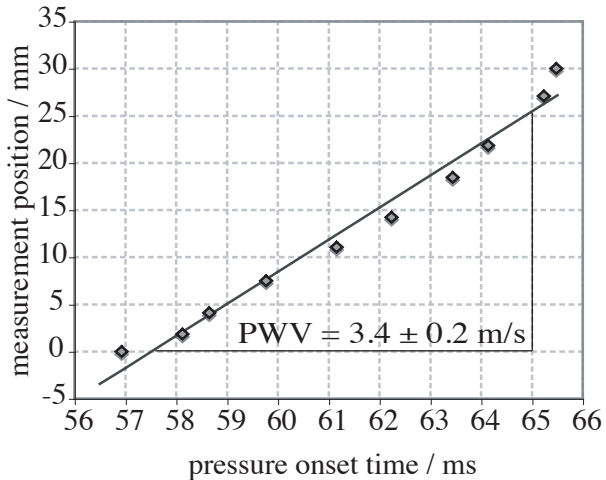
b) catheter position vs. pressure onset time
