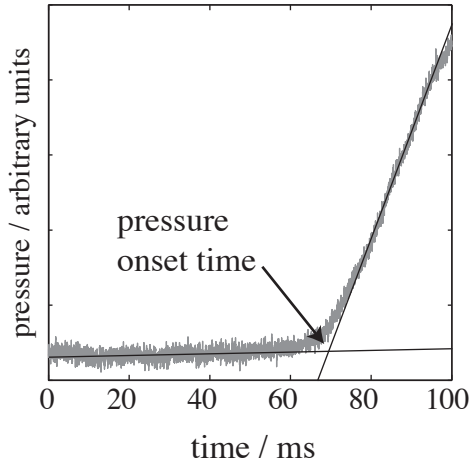
a) recorded pressure pulse wave
