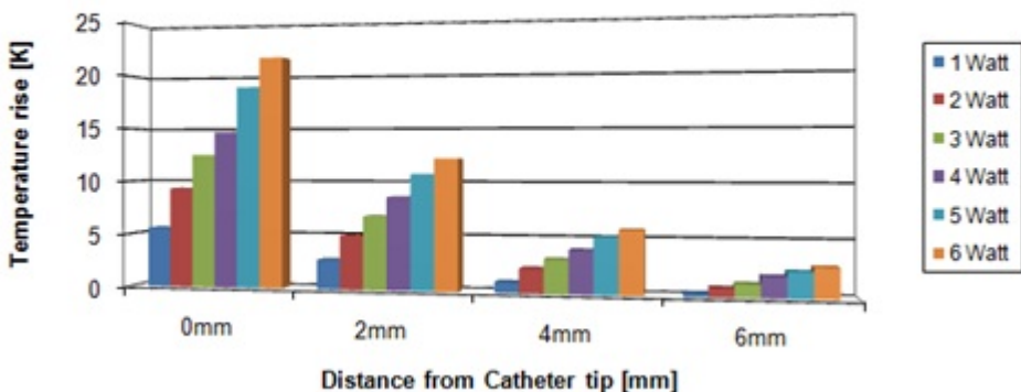
Temperature distribution with increasing tissue depth - measured at six power levels and with low contact force (10g)
