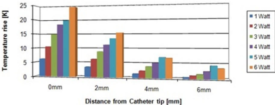
Temperature distribution with increasing tissue depth - measured at six power levels and with high contact force (90g)
