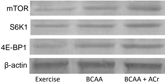
Supplementary Figure 1. Western Blot bands for mammalian target of rapamycin (mTOR), ribosomal protein S6 kinase beta-1 (S6K1), eukaryotic translation initiation factor 4E-binding protein 1 (4E-BP1), and \beta -actin levels.
