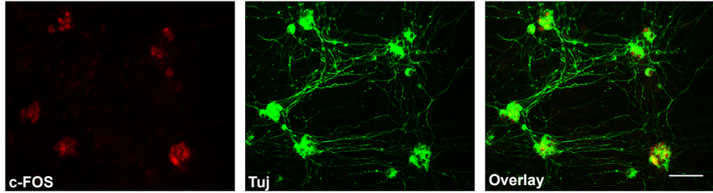
Immunocytochemical double labeling of rENSpc were performed using anti-c-Fos (Calbiochem) and anti-Tuj ( \beta III-tubulin; Sigma) antibodies after 7 hours of EFS. Scale bar : 50 \mu m.
