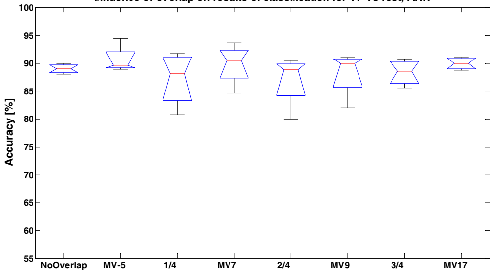
Influence of overlap on results of classification for VF vs rest, ANN
