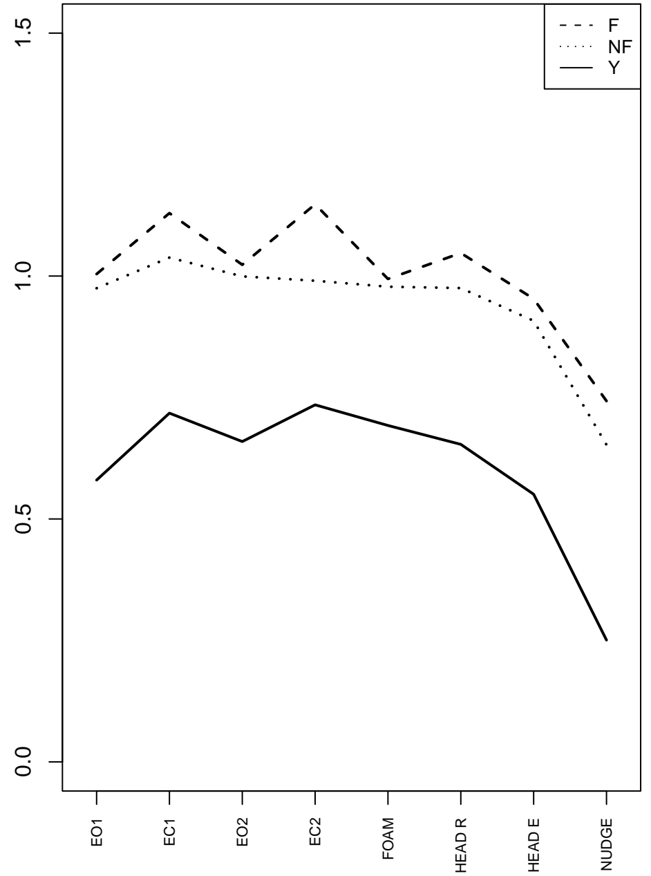
Entropy S(Y)
