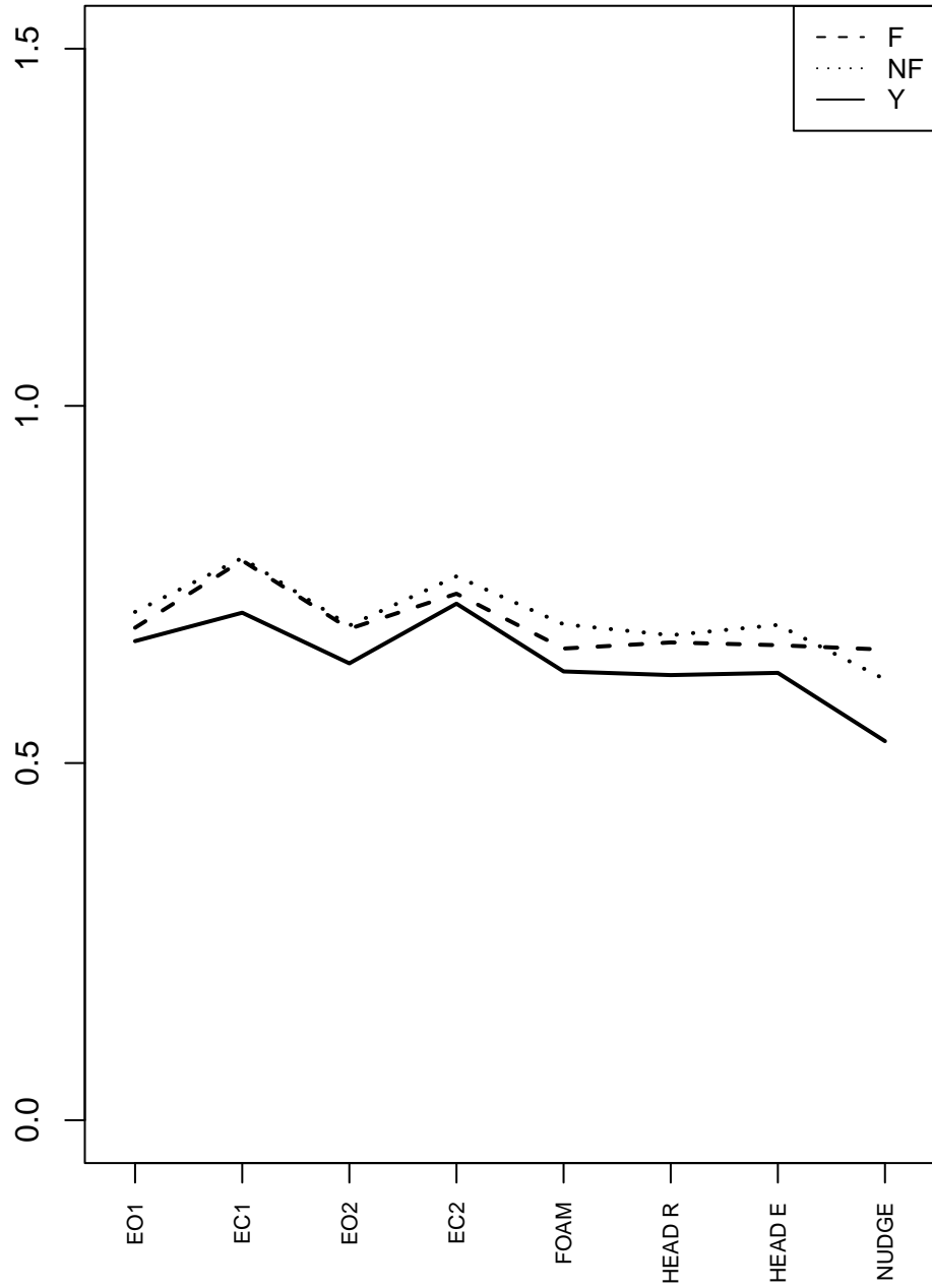
Entropy S(X)
