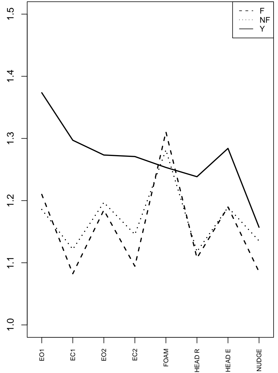
Hurst ss-exponent \alpha(Y)
