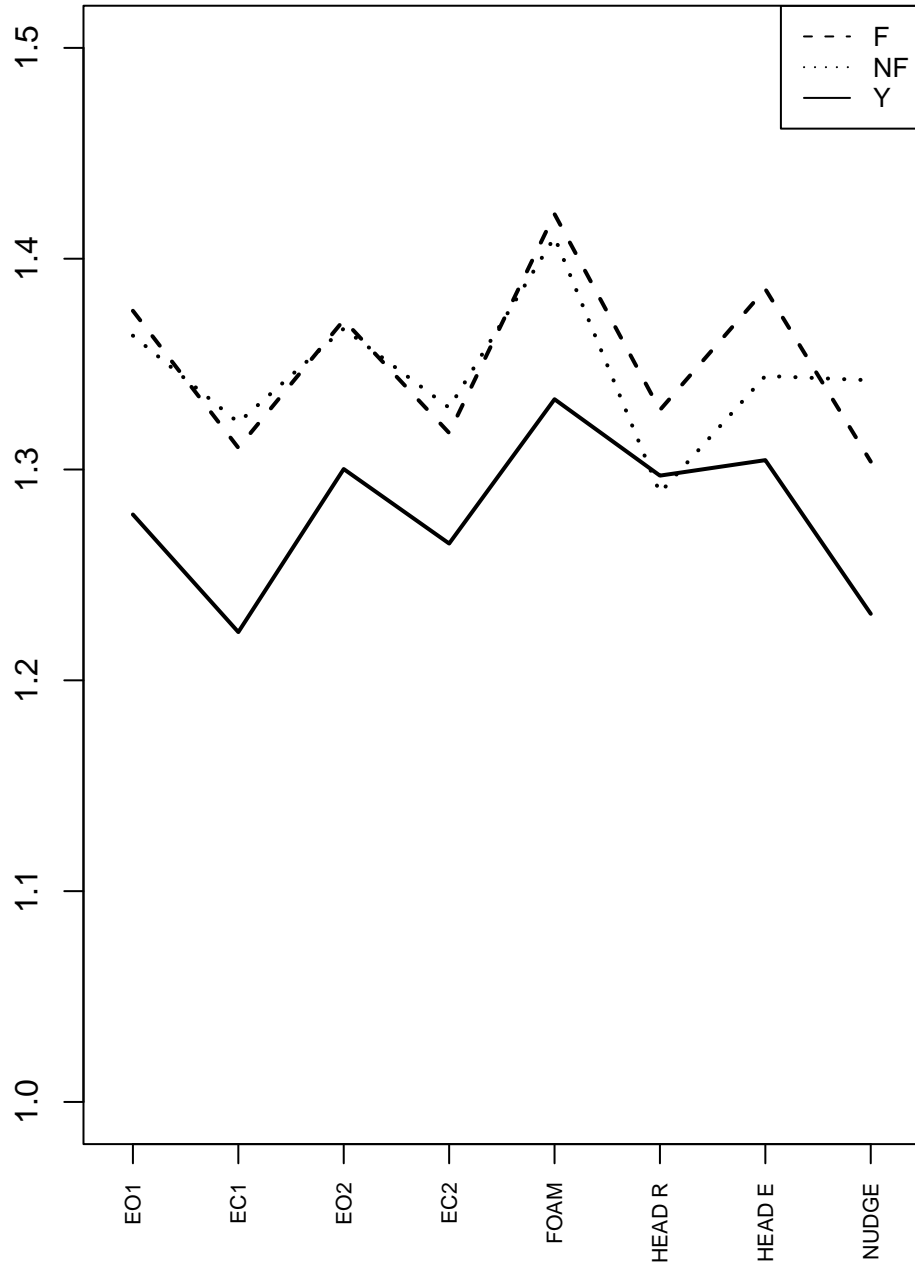
Hurst ss-exponent \alpha(X)
