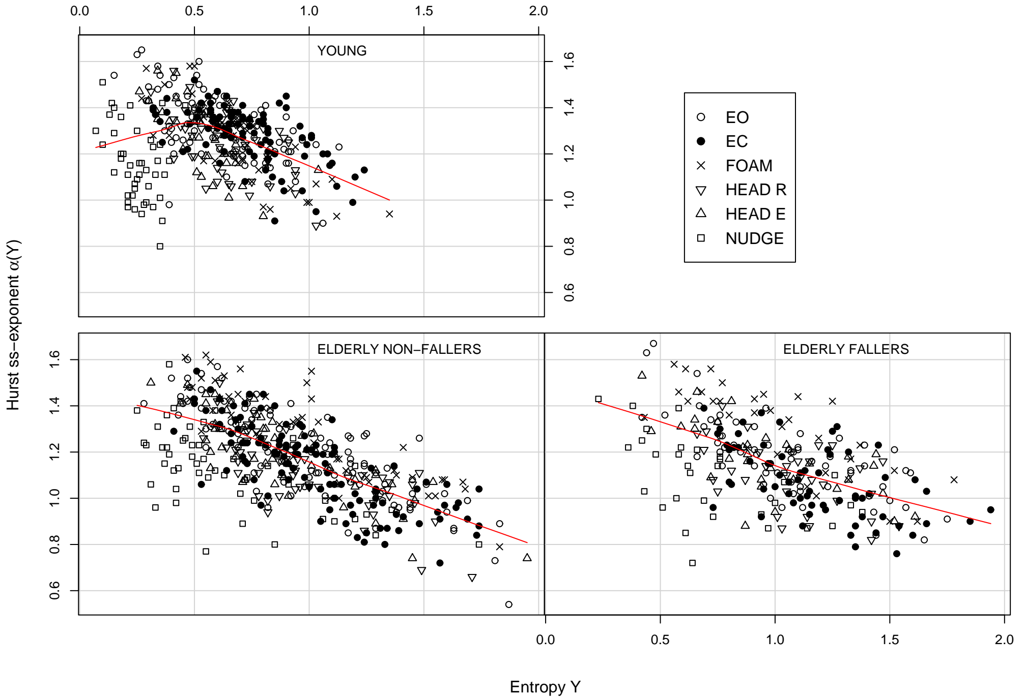
Hurst ss-exponent \alpha(Y) vs Entropy Y
