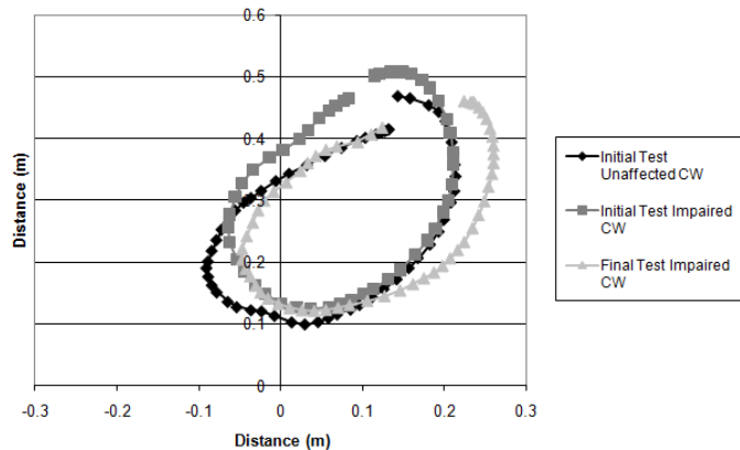
Big Circle Motion Test
