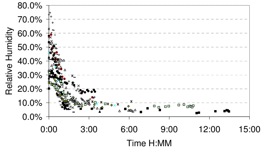
10B Flight Humidity Until Beginning of Descent
