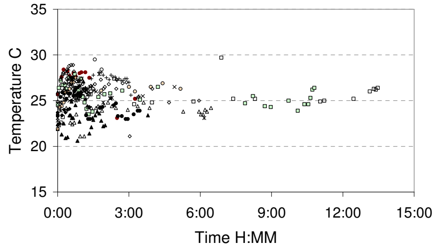
10A Flight Temperature Until Beginning of Descent
