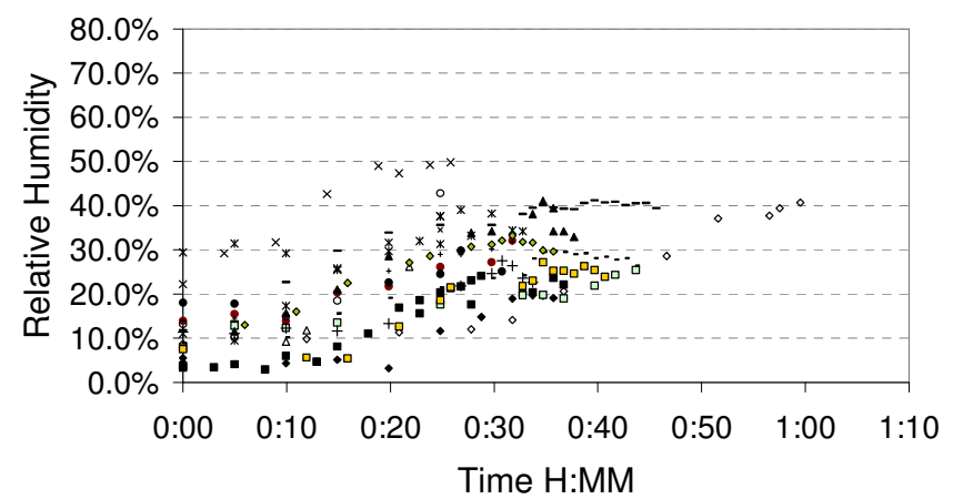
10D Flight Humidity From Beginning of Descent Until Gate
