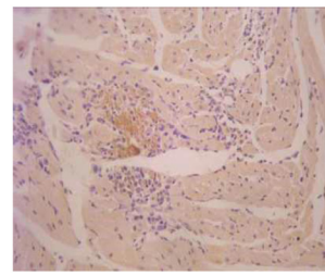
d: 21d (200×)
