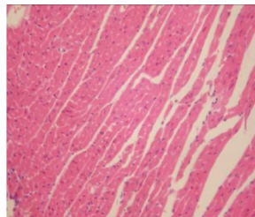
b: 3d (200×)
