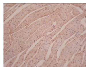
b: 3d (200×)
