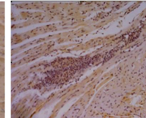
f: 55d (200×)
