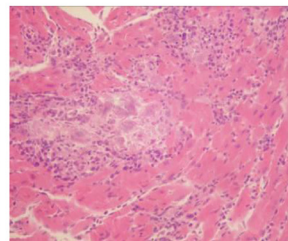
d: 21d (200×)
