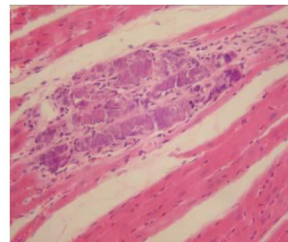
f: 55d (200×)
