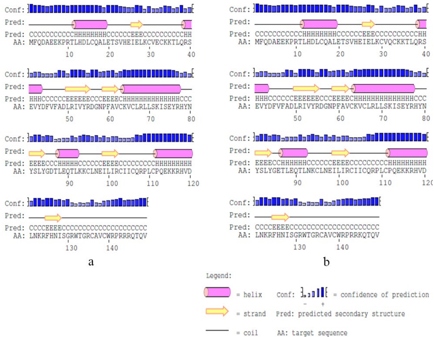
Figure S3. Secondary structure prediction of HPV-58 E6 reference and variant sequence
