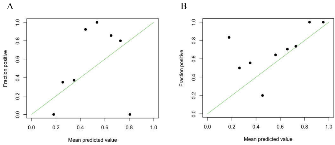
Figure S1. : Reliability diagram for SLR without calibration (A), and calibrated SSVM using platt calibration (B).
