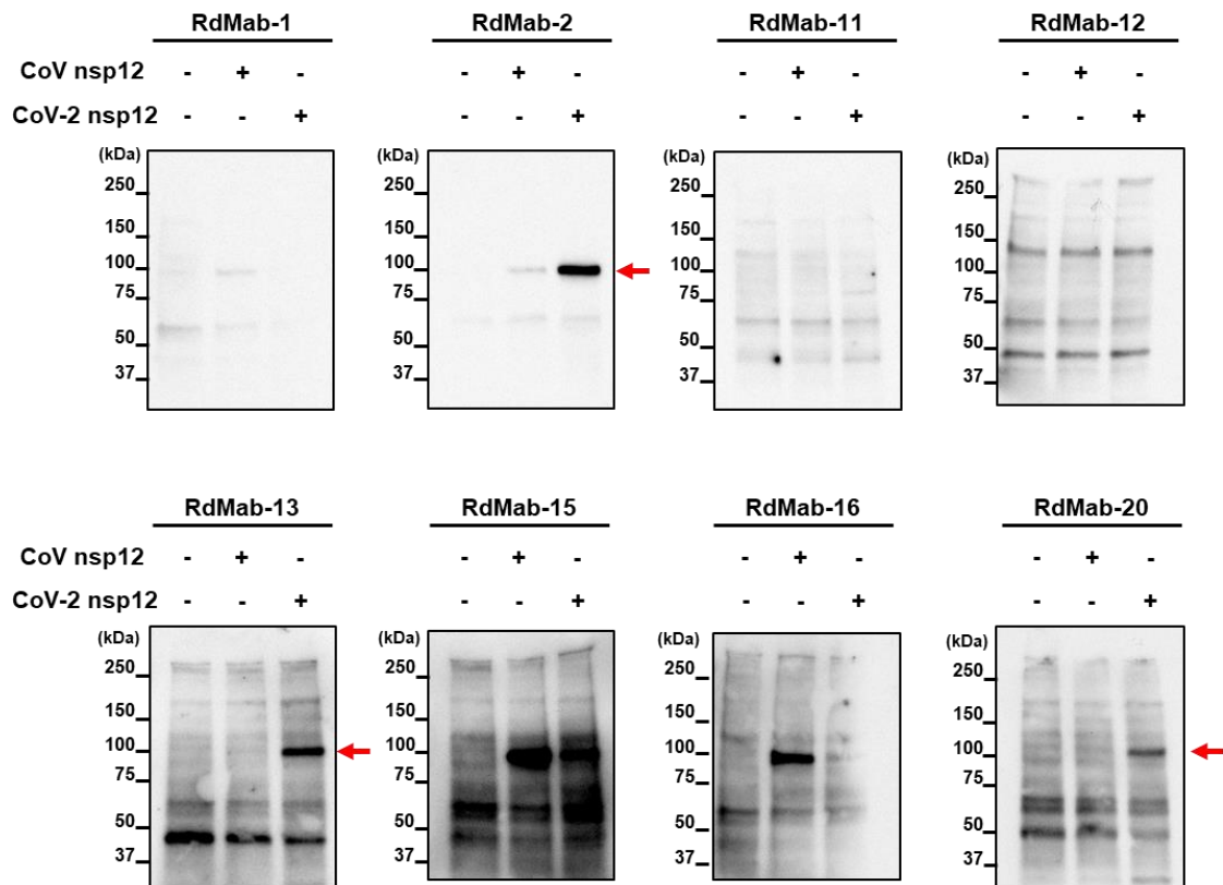
Fig. S2. Selection of anti-nsp12 mouse monoclonal antibodies to discriminate between nsp12 of SARS-CoV and SARS-CoV-2
