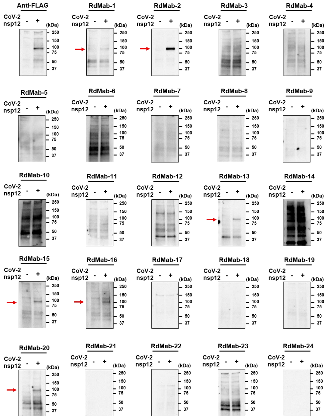
Fig. S1. Screening of anti-nsp12 mouse monoclonal antibodies using the culture supernatant of hybridomas
