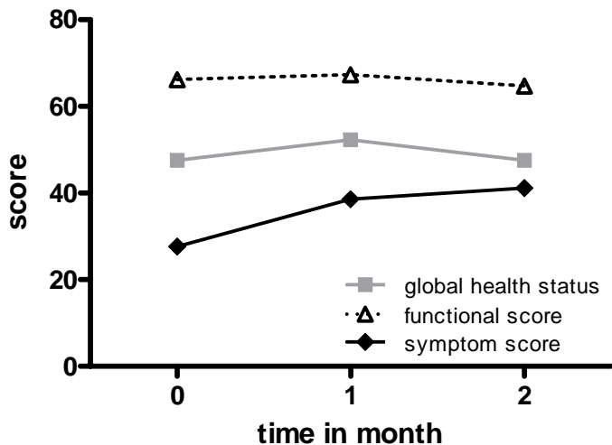
global scores
