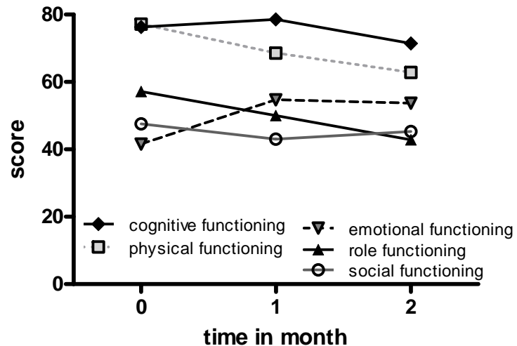
functional scores
