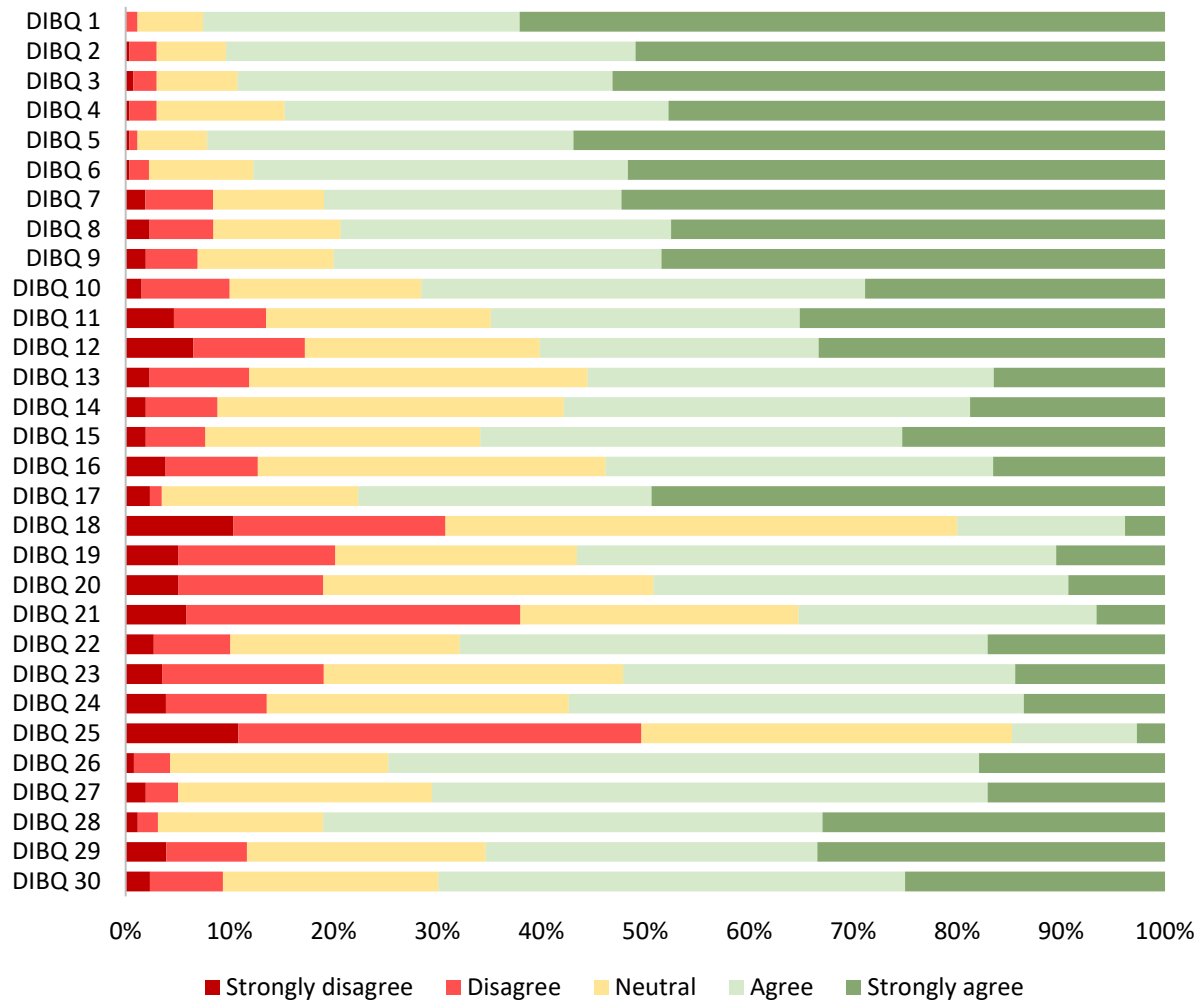
Distribution of responses to individual items of the modified DIBQ
