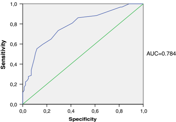
ROC Curve of Sodium concentration
