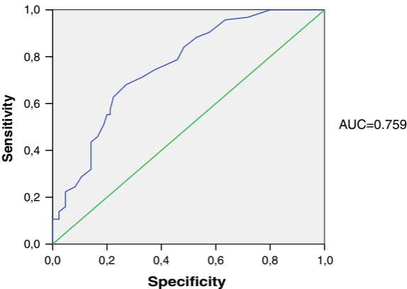
ROC Curve of Chloride concentration
