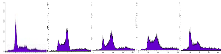
SAS/mp53
