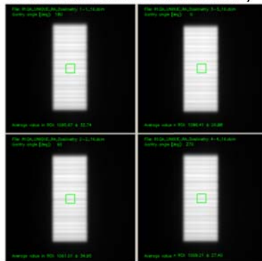
Test 3: accurate control of leaf speed during RapidArc delivery
