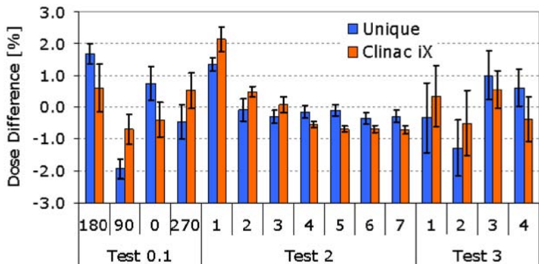
Test 2: Accurate control of dose rate and gantry speed during RapidArc delivery
