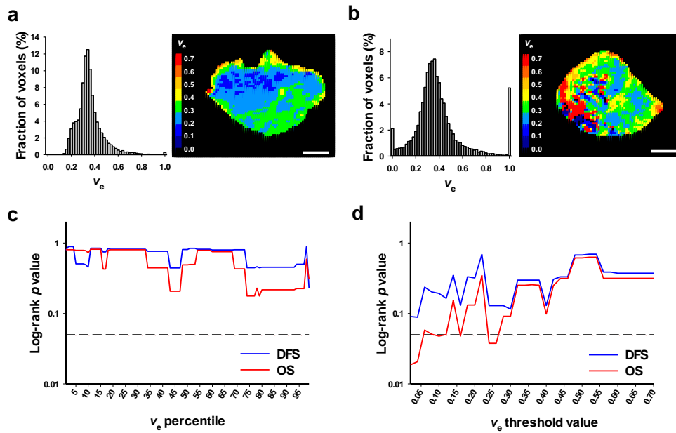
Additional file 1: Figure S1. Analysis of v_e data. Parametric v_e image and v_e frequency distribution of a high-enhancing tumor a and a low-enhancing tumor b , and plots of log-rank p value versus v_e percentile c and log-rank p value versus v_e threshold value d . Scale bars: 1 cm.
