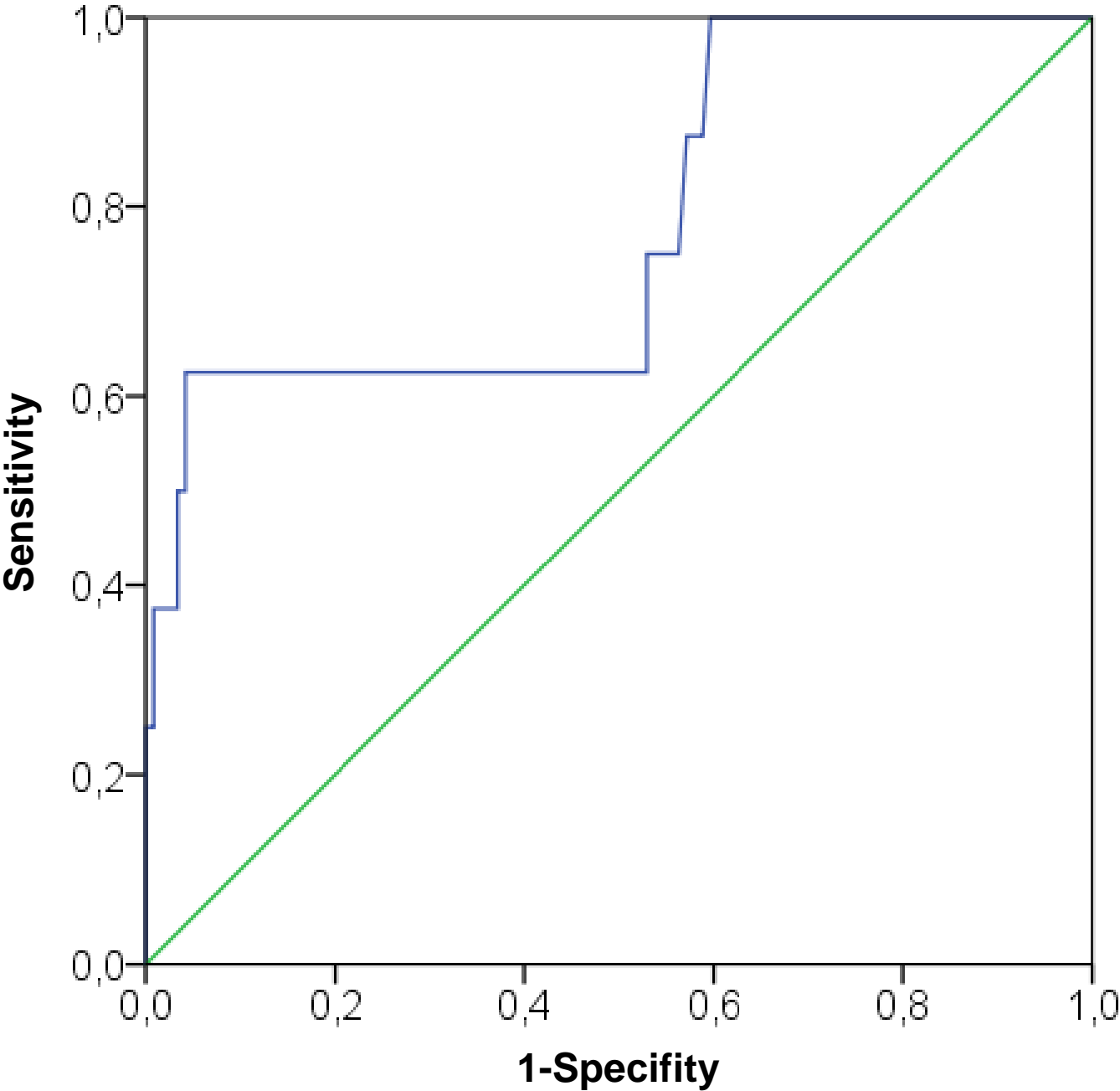
ROC-Curve
