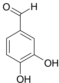
Protocatechualdehyde
