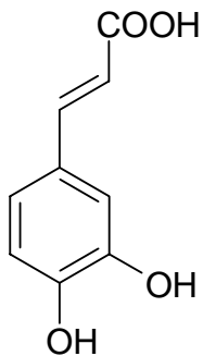
Caffeic acid
