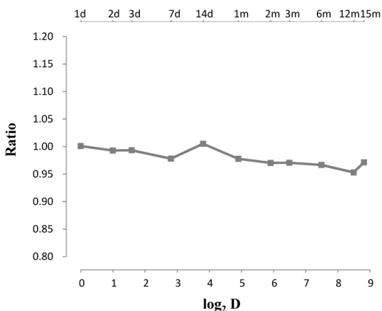
Berberine
