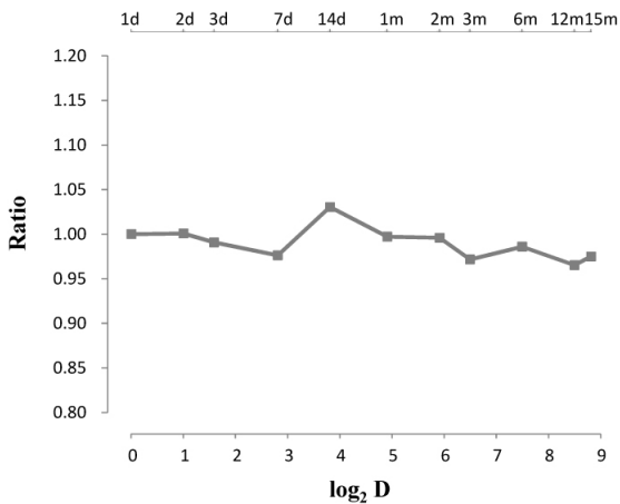
Hesperidin
