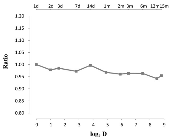
Palmatine
