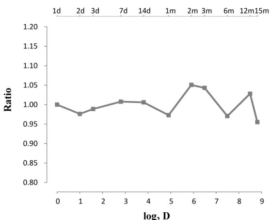
Schisandrin
