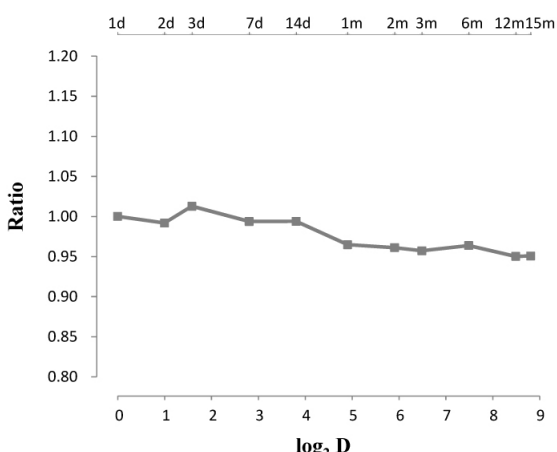
Magnolol
