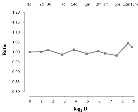
Aesculetin
