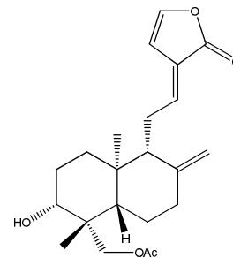
19-O-acetylanhydroandrographolide
