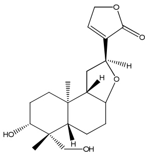
isoandrographolide
