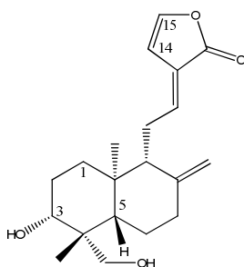
14-deoxy-14,15-didehydroandrographolide
