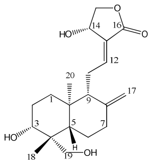
andrographolide
