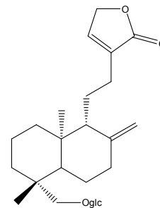
neoandrographolide
