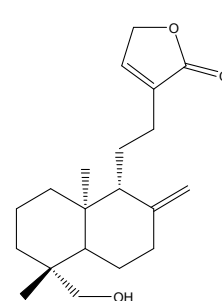
andrograpanin
