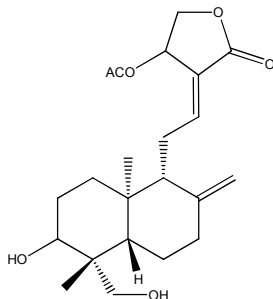
14-acetylandrographolide
